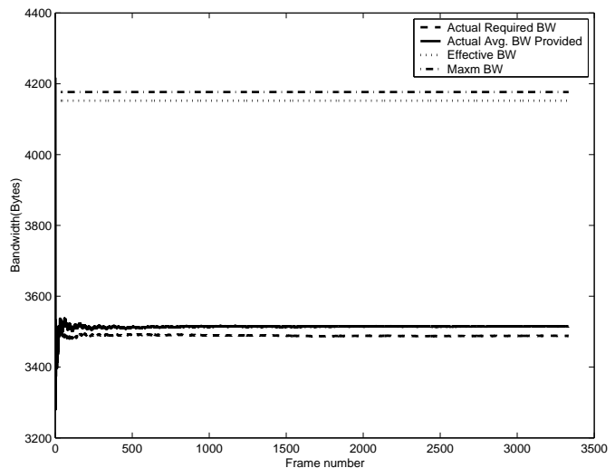
Figure 5: Comparison of Bandwidth required and Bandwidth provided
